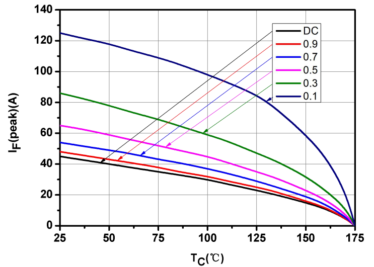
Fig.8-Current Derating
