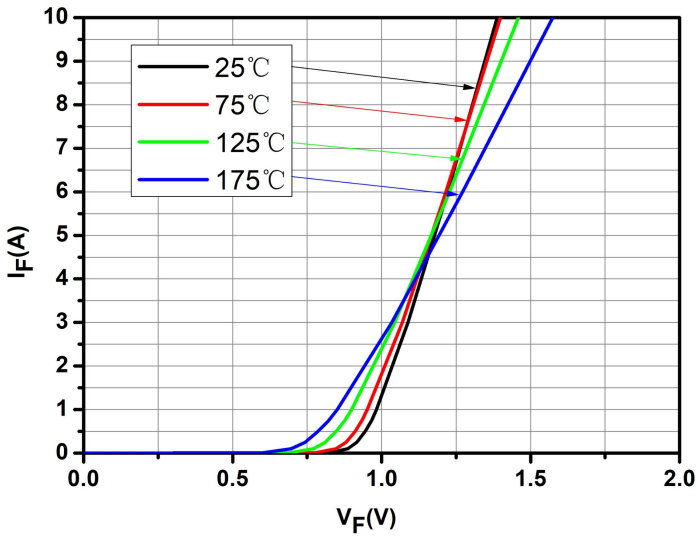
Fig.1-Typical Forward Voltage
